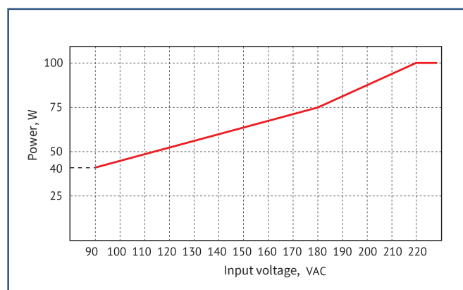
Power dependence on input voltage at tmin for version "P"
